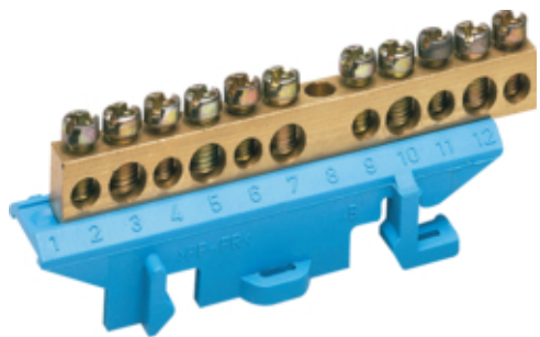
Brass terminal, 5x10mm 2 5x16mm 2 , N
